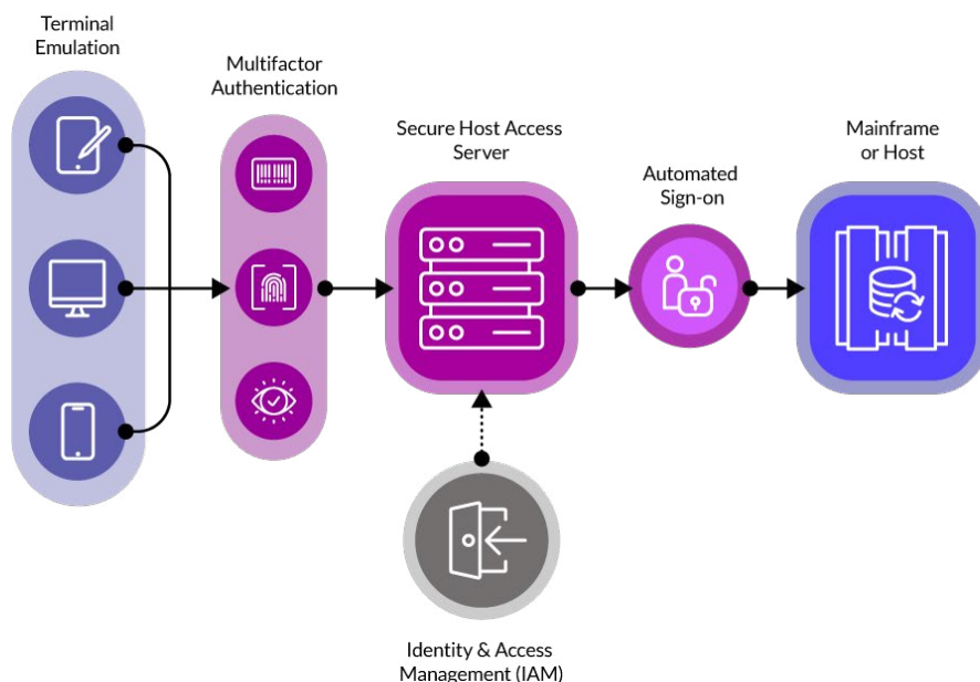
Figure 1. Users no longer need to take the additional step of entering a password to log on to their host applications after authenticating to Rocket Secure Host Access. The Rocket tool handles that for them.
